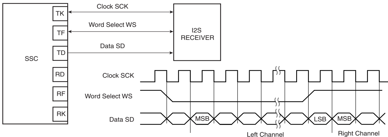
Figure 32-16. Audio Application Block Diagram
