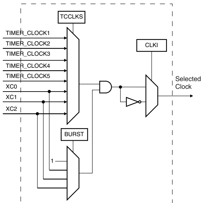
Figure 33-2. Clock Selection
