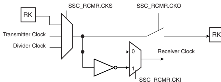
Figure 32-7. Receiver Clock Management
