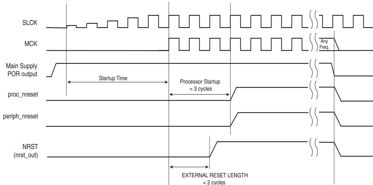
Figure 14-4. Power-up Reset
