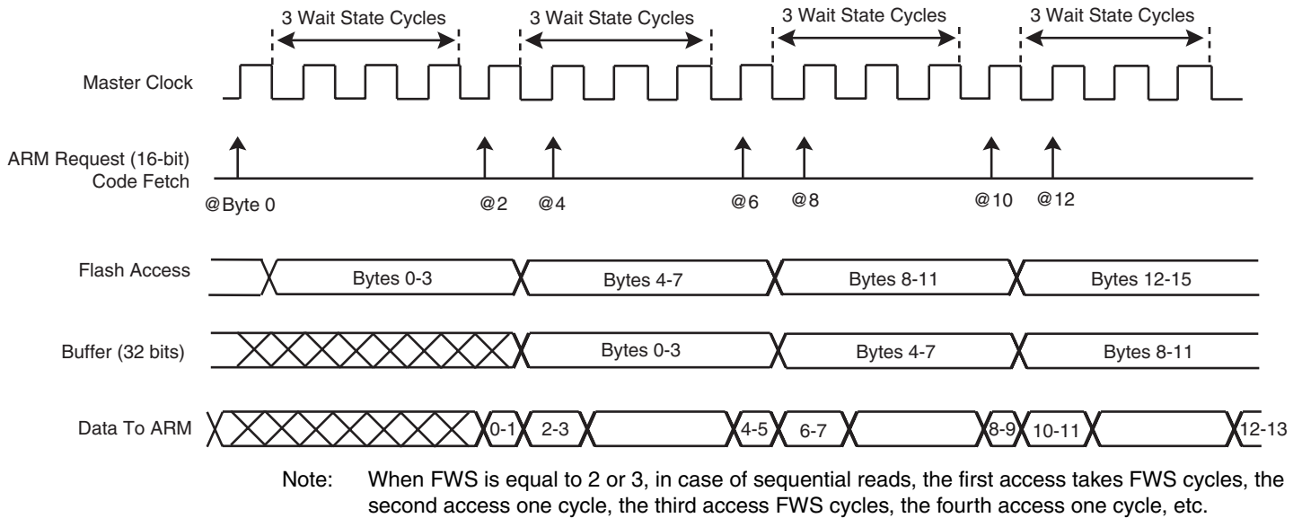
Figure 20-4. Code Read Optimization in Thumb Mode for FWS = 3
