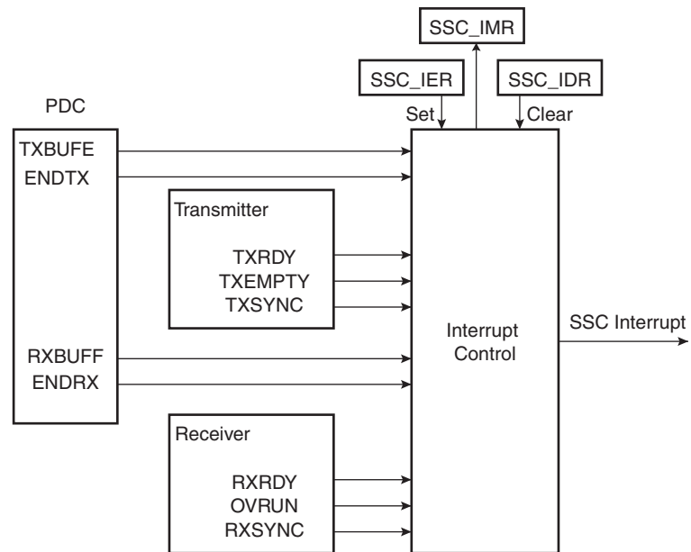
Figure 32-15. Interrupt Block Diagram
