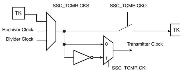
Figure 32-6. Transmitter Clock Management
