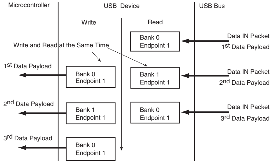
Figure 35-9. Bank Swapping in Data OUT Transfers for Ping-pong Endpoints
