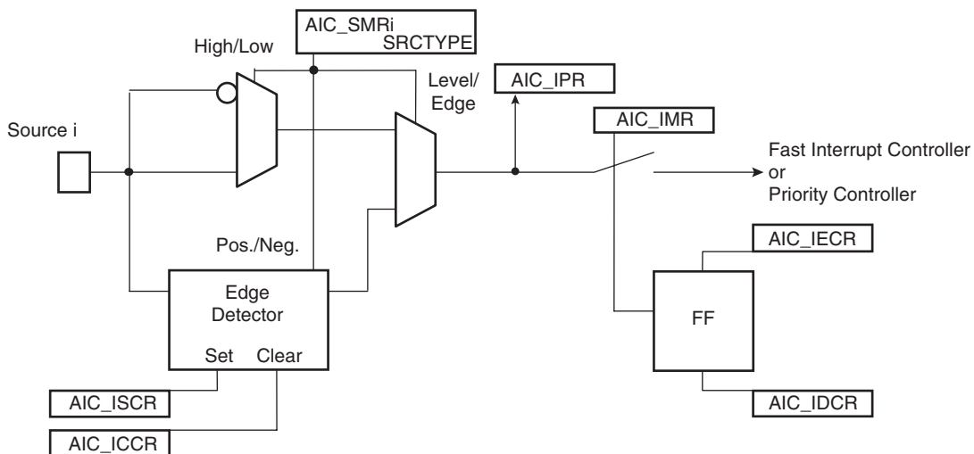
Figure 24-5. External Interrupt Source Input Stage
