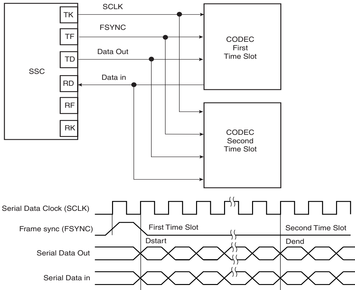
Figure 32-18. Time Slot Application Block Diagram
