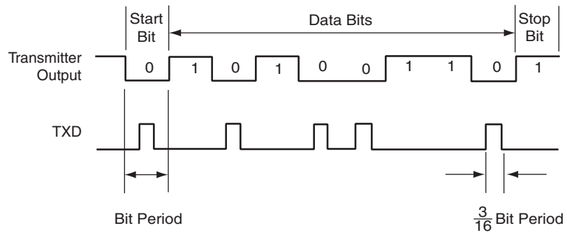
Figure 31-36. IrDA Modulation
