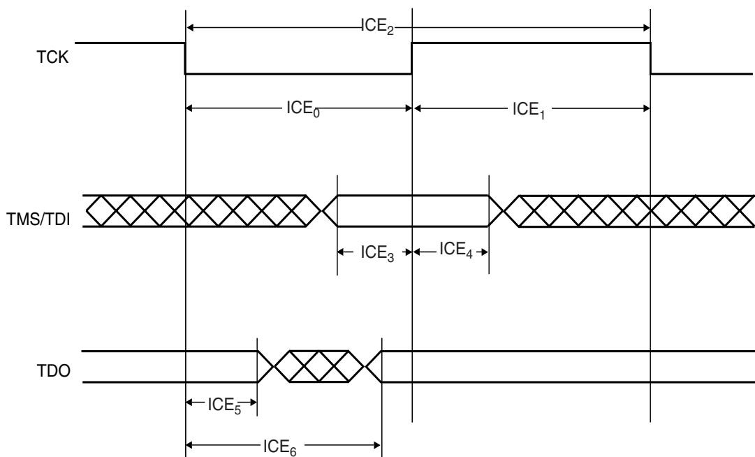
Figure 37-7. ICE Interface Signals
