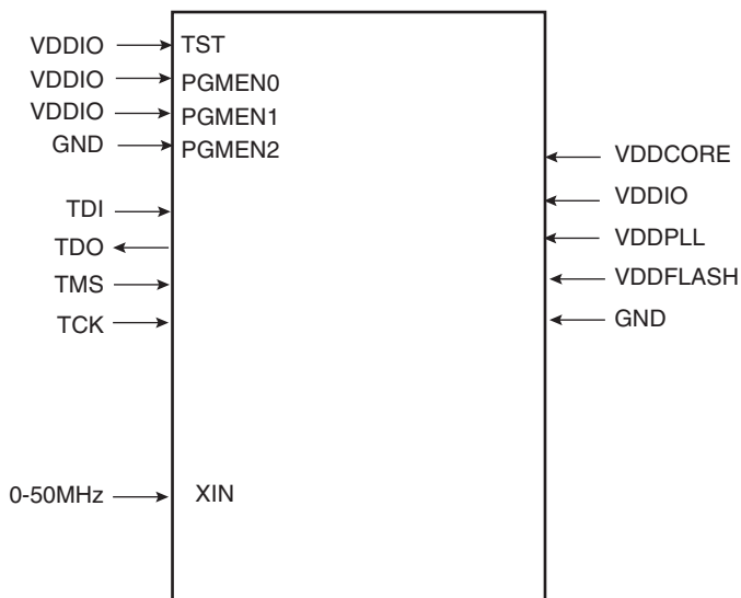
Figure 21-7. Serial Programming
