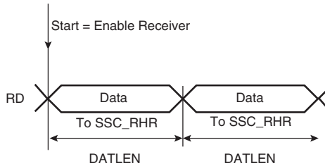
Figure 32-14. Receive Frame Format in Continuous Mode
