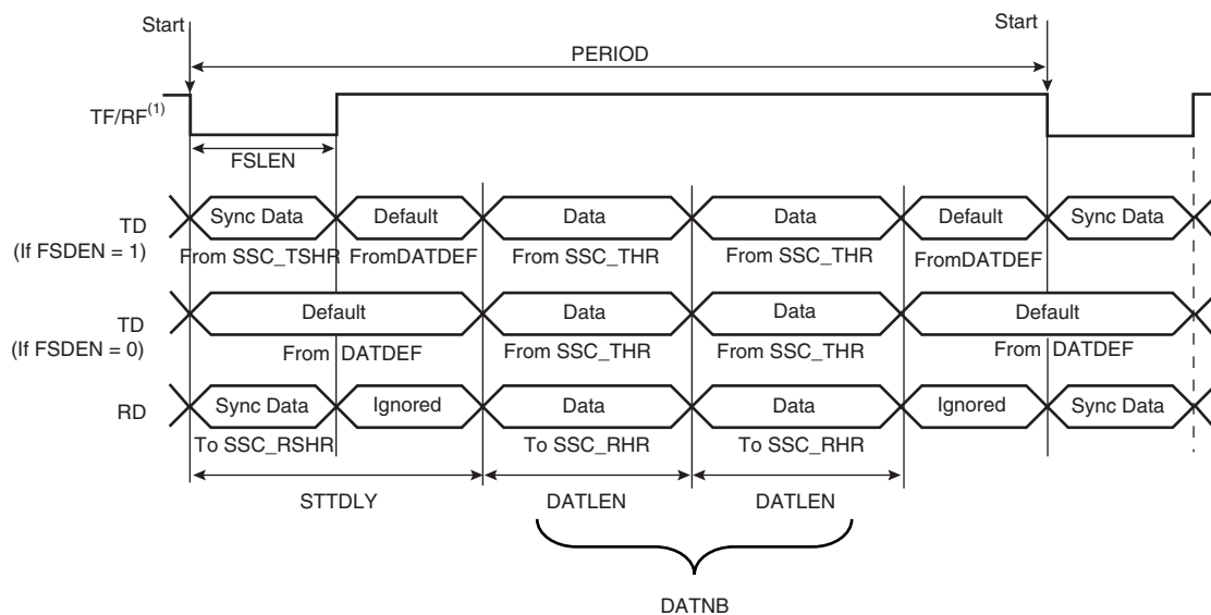
Figure 32-12. Transmit and Receive Frame Format in Edge/Pulse Start Modes
