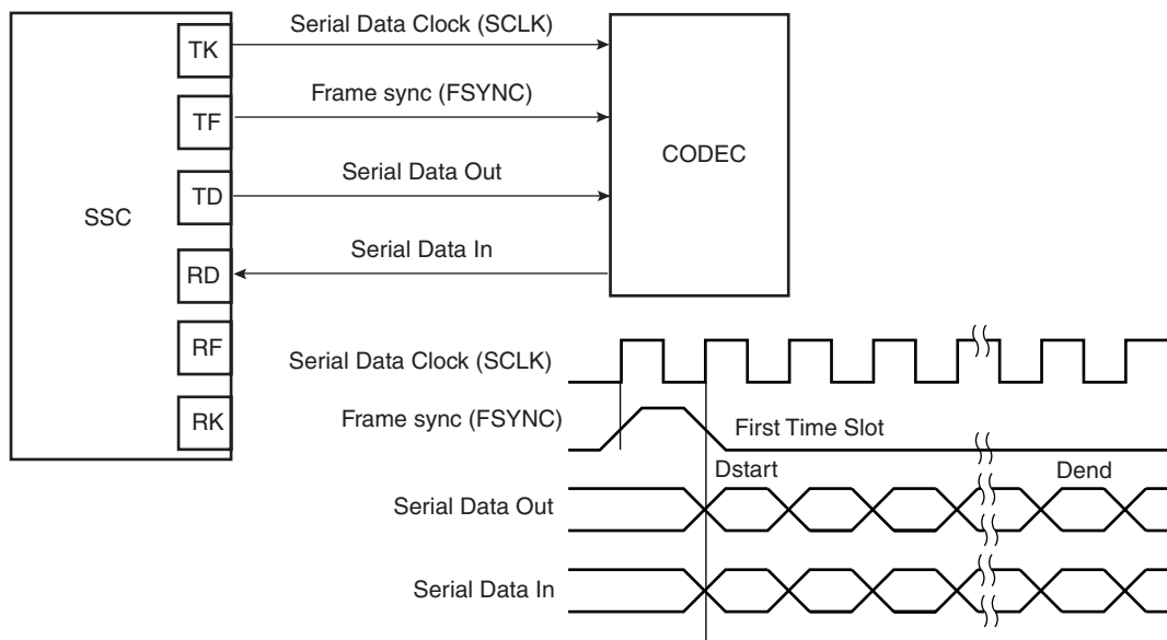
Figure 32-17. Codec Application Block Diagram
