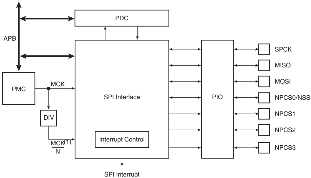
Figure 29-1. Block Diagram
