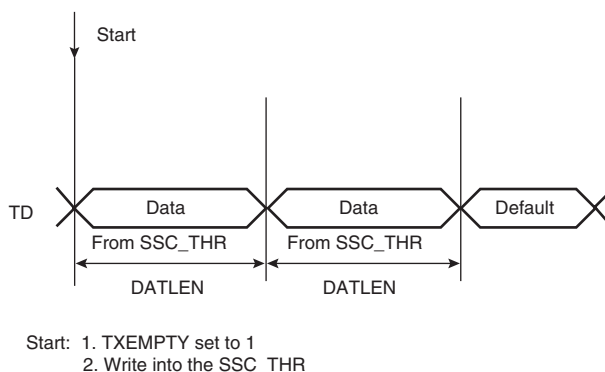
Figure 32-13. Transmit Frame Format in Continuous Mode
