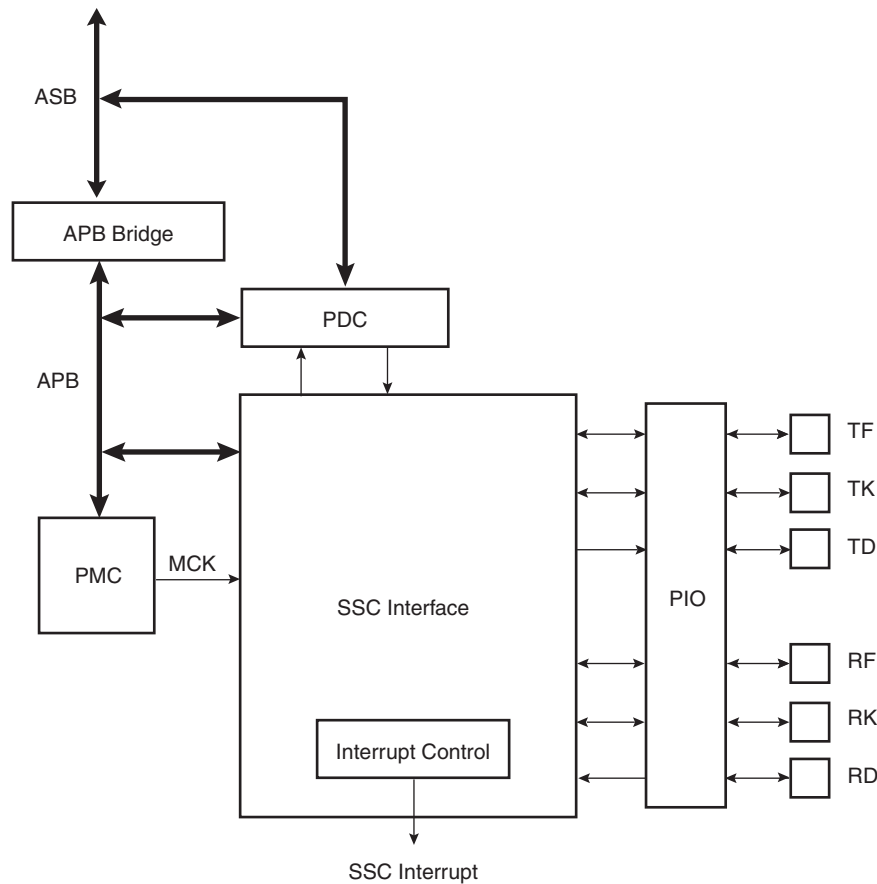
Figure 32-1. Block Diagram
