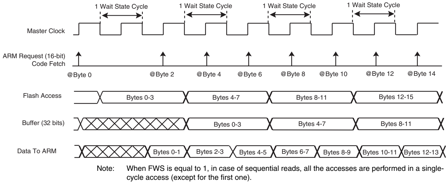
Figure 20-3. Code Read Optimization in Thumb Mode for FWS = 1
