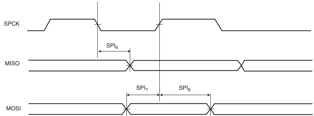
Figure 37-5. SPI Slave mode with (CPOL=0 and NCPHA=0) or (CPOL=1 and NCPHA=1)
