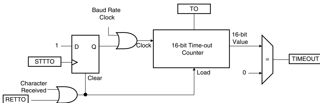
Figure 31-26. Receiver Time-out Block Diagram
