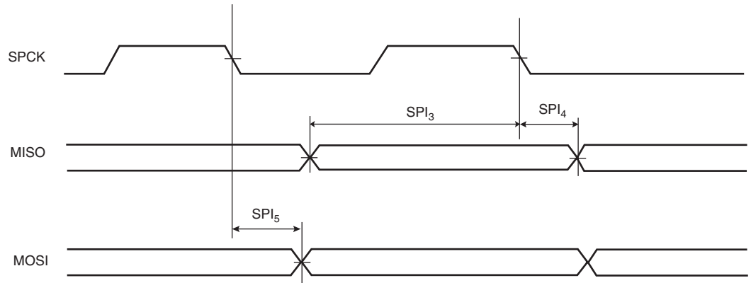
Figure 37-4. SPI Master mode with (CPOL=0 and NCPHA=0) or (CPOL=1 and NCPHA=1)
