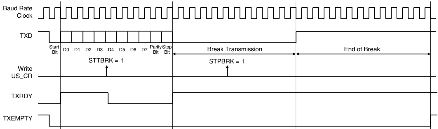
Figure 31-28. Break Transmission
