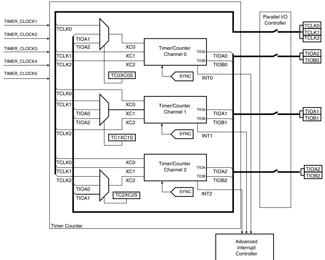
Figure 33-1. Timer/Counter Block Diagram (1)
